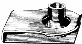
Part# 43566 "U" Nut for Pick-up Beds & Bumper Bracket M12-1.75, Throat: 42.5mm, PR 3.0-7.0 Aluminum Oxide Finish Ford Ranger, Dodge Durango Unit Package: 5
