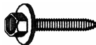
Part# 44343 M6 - 1.00 x 35mm 10mm Indented Hex Head 17mm O.D. Loose Washer Black Phosphate Finish Metric Type CA Body Bolts Unit Package: 25
