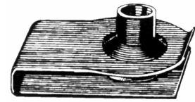
Part# 43321 Long Extruded "U" Nuts M6-1.0 Screw Size Panel Range: .34mm - 4.0mm Center of Hole to Edge: 19.5mm Unit Package: 25
