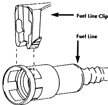
Part# 47210 Fuel Line Retainer Clip Fits 5/16" Fuel Line Unit Package: 25
