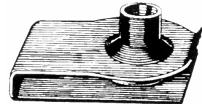
Part# 43324 Long Extruded "U" Nuts M8 - 1.25 Screw Size Panel Range: .80mm - 4.50mm Center of Hole to Edge: 20mm Unit Package: 25
