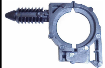
Part# 47164 Wire Loom Routing Clip For 1/2" ID, 11/16" OD Loom Stem Diameter: 3/8" x 2-1/2" Stem Length: 1/2" Fits Into 1/4" Hole Unit Package: 15
