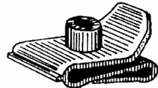
Part# 43336 Plastic "U" Nuts #10 Screw 20mm x 31mm Unit Package: 15
