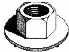
Part# 43210 8-1.25mm Metric Hex Nuts 13mm Hex Size 24mm O.D. Loose Barbed Washer Black Phosphate Finish Unit Package: 25
