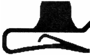
Part# 43340 Extruded "U" Nuts 10 - 1.50mm Panel Range: .035" - .232" Center of Hole to Edge: 3/4" Black Phosphate Finish Unit Package: 25
