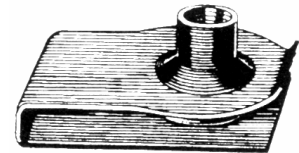
Part# 43568 "U" Nut Rear Bumper Bracket M12-1.75 Throat: 33.5 mm, PR: 1.5 - 5.5 Black Organic & Oil Finish GM C/K Trucks Unit Package: 5
