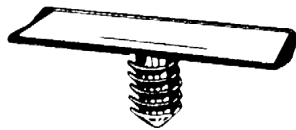
Part# 47162 Nylon Rear Light Wiring Retainer 3/8" Wide, 1-7/16" Long Stem: 9/32" x 7/16" Long Unit Package: 50
