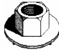
Part# 43223 M5 Nut - .80 w/19mm Free Spinning Washer Black Finish Unit Package: 25
