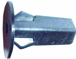
Part# 48489 Splash Shield Retainer Toyota X-Long Unit Package: 15
