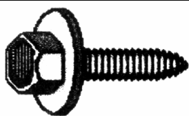
Part# 44344 M6 x 1.00 x 25mm 10mm Indented Hex Head 17mm O.D. Loose Washer Black Phosphate Finish Metric Type CA Body Bolts Unit Package: 50
