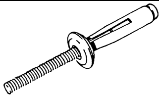
Part# 42220 Blind Type Rivet 1/4" Rivet with 1/2" Flange .120 - .400 Grip Range Unit Package: 15
