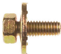
Part# 44104 M6 - 1.00 x 16mm 10mm Indented Hex Head 18.5mm O.D. Loose Washer Zinc and Yellow Finish Metric Type Body Bolts GM 11503812 Unit Package: 50
