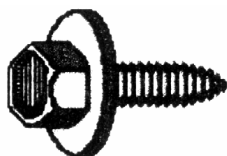
Part# 44347 M6 - 1.00 x 20mm 10mm Indented Hex Head 17mm O.D. Loose Washer Black Phosphate Finish Metric Type CA Body Bolts Unit Package: 50
