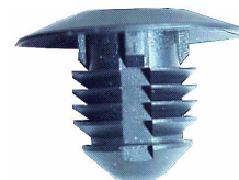
Part# 47468 12.5 Hole Retainer Jeep, Trailblazer, Chrysler Unit Package: 25
