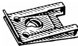
Part# 43332 #8 Screw Size Panel Range: .025" - .150" Center of Hole to Edge: 5/8" Long Unit Package: 100
