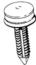
Part# 47216 GM Door & Trim Panel Clip Hole Diameter: 7mm 30mm O/L Unit Package: 50
