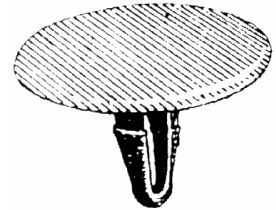
Part# 48443 Toyota Retaining Clip Head Diameter: 30mm Stem Length: 17mm Hole: 7mm, Panel: 6mm Unit Package: 25
