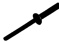
Part# 42218 Closed End Sealing Type 1/8" Diameter Grip Range: 3/16"-1/4" 7/32" Flange (Black) Aluminum Luggage Racks Unit Package: 50
