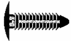
Part# 47315 1/4" Hole Size Panel Range: .095" - .805" Black Nylon Shield Retainers Unit Package: 50
