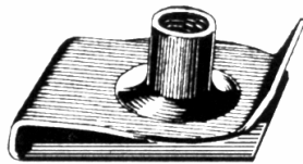
Part# 43322 Phosphate Short Extruded "U" Nuts M6 - 1.0 Screw Size Panel Range: .80mm - 4.0mm Center of Hole to Edge: 13.5mm Unit Package: 25
