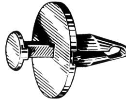
Part# 47307 Black Nylon Spare Tire Clip Head Diameter: 1" Fits Into 5/16" Hole Unit Package: 25
