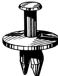
Part# 47106 Fascia Retainer Head Diameter: 1" Panel Range: 1/4" Fits Into 3/8" Hole Unit Package: 25
