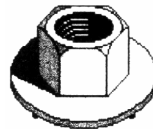
Part# 43335 6 - 1.00mm 10mm Hex Size 16mm O.D. Loose Barbed Washer Black Phosphate Finish Metric Hex Nuts GM Unit Package: 50
