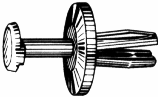
Part# 47309 Nylon Front Fender Mud Skirt Retainer Head Diameter: 11/16" Panel Range: 9/32" Fits Into 1/4" Hole Unit Package: 25
