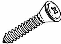
Part# 45281 Phillips Oval Head Trim Screws With Flush Washer Type AB Black Phosphate #8 x 1" With #6 Head Unit Package: 50
