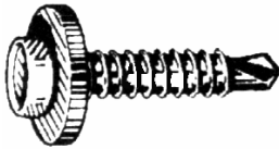
Part# 45101 M4.2 - 1.41 x 20mm (#8 x 25/32") Black Hex Head Sems® With Teks® Point 12mm (1/2") Washer O.D. 7mm Hex Unit Package: 50
