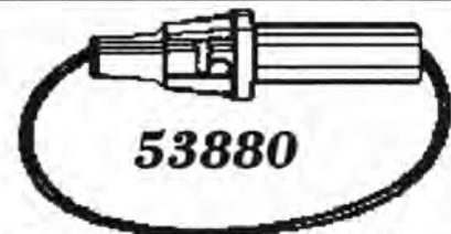
53880 TWIST-LOCK FUSE HOLDER FOR USE UP TO 20 AMPS. SUPPLIED WITH 14 AMP FUSE 16 GAUGE WIRE
