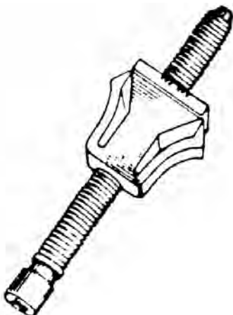
Part# 46212 White Headlamp Adjusting Screw & Nut Assembly 1/4" - 28 x 2" Screw GM Unit Package: 25
