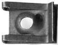
Part# 43572 Short U Nuts Black Phosphate Finish #14 Screw Size Panel Range: .025 — .150 Center: 3/8 Unit Package: 50
