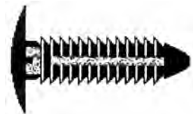
Part# 47315 1/4" Hole Size Panel Range: .095" - .805" Black Nylon Shield Retainers Unit Package: 50
