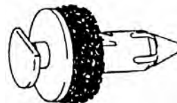
Part# 47449 Door & Tail Gate Trim Retainer Hole: M8, Stem: 18mm, PR: 8-1.5mm Chrysler Mini Vans & Dodge Durango Unit Package: 15
