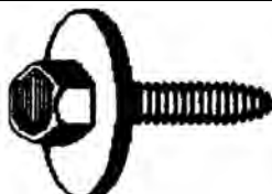
Part# 44345 M6 - 1.00 x 25mm 10mm Indented Hex Head 24mm O.D. Loose Washer Black Phosphate Finish Metric Type CA Body Bolts Unit Package: 50
