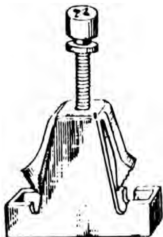
Part# 46214 Blue Nut Screw Size 12 28 x 1-3/4" Headlamp Adjusting Screw & Nut Assembly GM Unit Package: 25
