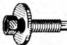
Part# 44342 M6 - 1.00 x 28mm 8mm Indented Hex Head 19mm O.D. Loose Washer Black Dichromate Finish Metric Dog Point Body Bolts Ford Head Unit Package: 50
