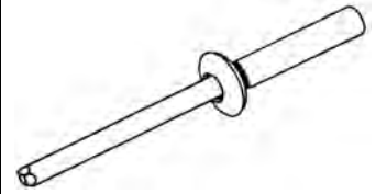
Part# 42213 Closed End Sealing Type (Black) Aluminum Rivet Aluminum Rivet 3/16" Rivet w/3/8" Flange Grip Range: .376-.500 Luggage Racks Unit Package: 25
