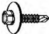
Part# 45337 4.2 - 1.41 x 20mm 7 mm Indented Hex Head 17mm O.D. Loose Washer Black Phosphate Finish Teks® Screws Unit Package: 50
