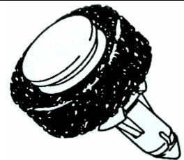
Part# 47446 Door Panel Retainer Hole: M9, Head: 19.5mm O/L: 27.8mm GM B, G, H Bodies 2000 Unit Package: 10
