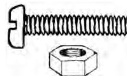
Part# 41108 Black Nylon M6-1.0 x 20mm Slotted Pan Head License Plate Screw & Nylon Nut 12mm Head Diameter 10mm Hex Width Unit Package: 100
