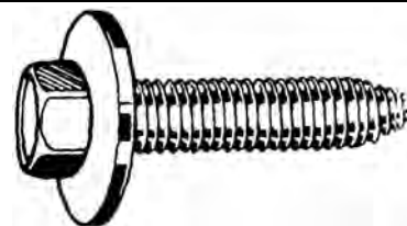
Part# 44103 M10 - 1.50 x 45mm Black Hex Head Sems Class 9.8 15mm Hex 30mm (1-3/16") Washer O.D. Unit Package: 10
