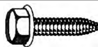
Part# 44346 M8 - 1.25 x 30mm 13mm Indented Hex Head 17mm O.D. Washer Black Organic Finish Metric Type CA Flange Bolts Unit Package: 25
