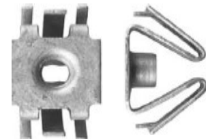
Part# 43229 Extruded Snap-in Type Nut License Plate, Fender, Sun Roof M6-1.0 Fits 13 x 20mm Hole Organic Zinc Phosphate Finish Unit Package: 10
