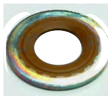
91101 Rubber Encased Metal Gaskets 12mm, GM Products 1982-up Replaces OEM# 14090908
