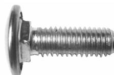
Part# 44349 8-1.25 x 25mm" Pan Head Stainless Steel Capped Bumper Bolts Unit Package: 25
