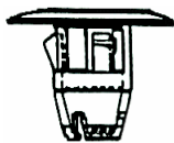
Part# 47447 Not Supplied by OEM Door Panel Retainer Grommet Hole: M9, PR: 1-1.75mm Flange: 19mm Chrysler LH 2000 Unit Package: 25
