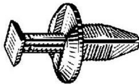
Part# 47157 Nylon Front Bumper Stone Deflector Retainer Head Diameter: 18mm Fits into 6.3mm Spare Hole Ford Unit Package: 25
