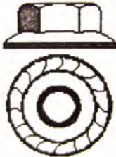
Part# 43342 8—1.25mm 13mm Hex Size 19mm O.D. Serrated Washer Black Phosphate Finish Metric Hex Flange Nuts Unit Package: 50
