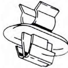
Part# 47163 Hood Prop Rod Clip Plastic Hole: 5 x 14mm Rectangular Slot Rod Diameter: 8mm Unit Package: 15
