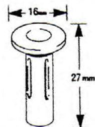
Part# 43226 Flat Head Rivet Style Nuts Steel Blind Hole Applications Leg Retention Style M6-1.0 Thread, 11mm Hole Unit Package: 5
