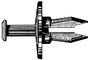
Part# 47305 Head Diameter: 1" Panel Range: 1/8" Fits Into 1/2" Hole Unit Package: 25
