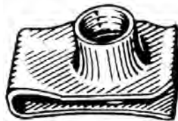
Part# 43323 Short Extruded "U" Nuts M8 - 1.25 Screw Size Panel Range: .80mm - 4.00mm Center of Hole to Edge: 14.5mm Unit Package: 25
